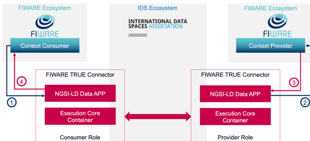
Figure 35 FIWARE TRUE Connector (source: fiware-true-connector.readthedocs.io )
